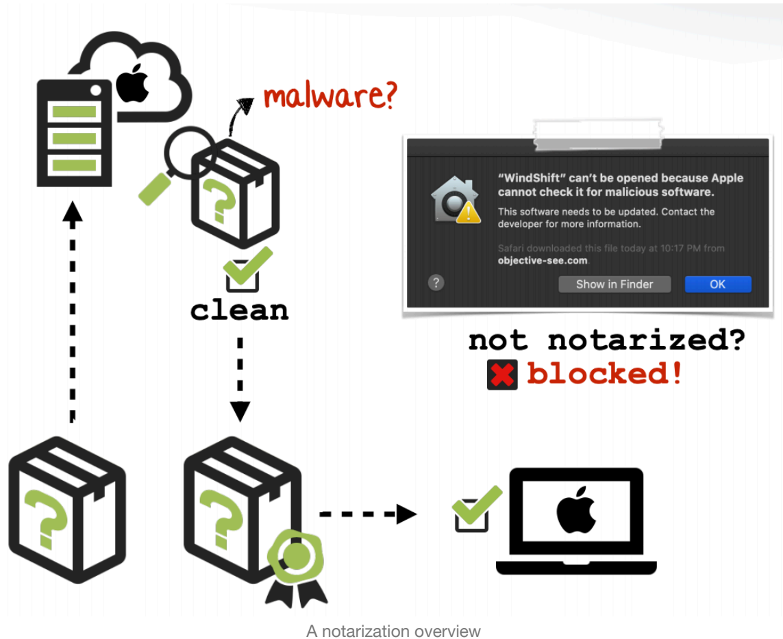
A notarization overview
